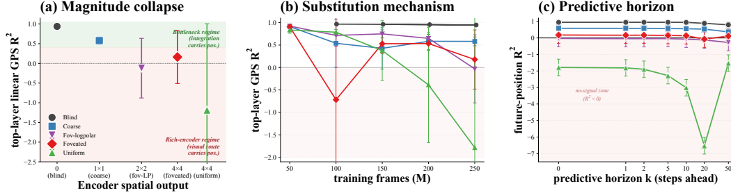
Figure 2: Three views of the magnitude axis. (a) Cross-condition : top-layer linear GPS R^2 falls with encoder bandwidth. (b) Across training : rich-encoder conditions start high then lose readability; bottleneck conditions hold it throughout. (c) Predictive horizon : only bottleneck conditions linearly decode \text{pos}_{t+k} at long k . Shaded band: R^2 < 0 , the linear probe is worse than predict-mean baseline — the “no-signal zone”. Uniform’s curve dives deep into this zone (its hidden state is scene-conditional, so 5-fold CV trains on some scenes’ position-directions and tests on incompatible ones, producing systematically negative R^2 ); the dive is noise, not a meaningful trend.
