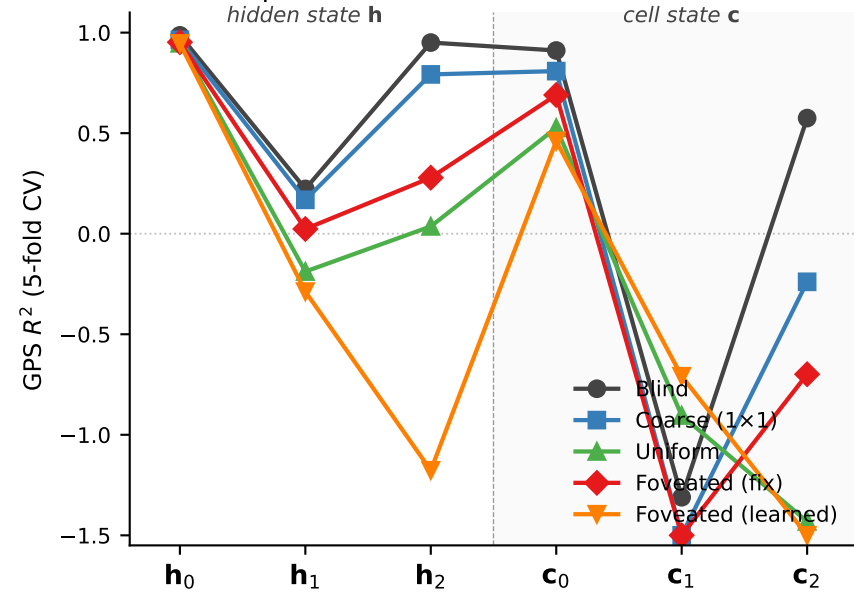
GPS probe across LSTM hidden + cell states
