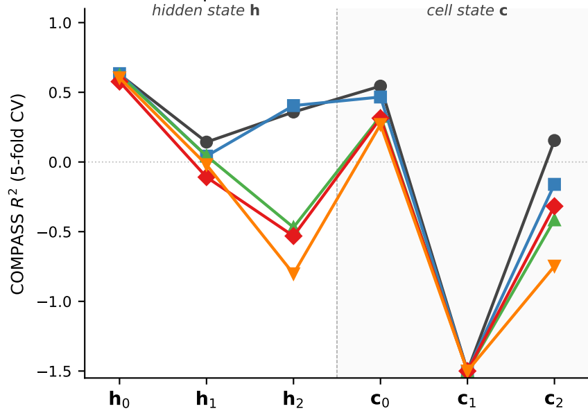
COMPASS probe across LSTM hidden + cell states
