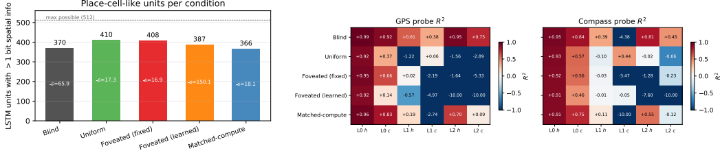
Figure 6: Left : LSTM units with > 1 bit spatial information per condition [Banino et al., 2018]; mean bits \bar{s} shown inside bars. Right : Per-layer, per-state linear probe R^2 for GPS (left sub-panel) and compass (right sub-panel) on deterministic-rollout hidden states. The multi-layer panel reveals an effect not visible at the top layer alone: even rich-encoder conditions (uniform, foveated, foveated-learned) carry world-frame spatial information at Layer 0 of the LSTM (closest to the visual encoder), with R^2 values comparable to blind/matched. The encoder-memory race is a per-layer phenomenon, not an all-or-nothing one — the deeper, top-layer state is what’s used by the policy and what we report in Table 1, and that is where the bottleneck conditions stand out.
