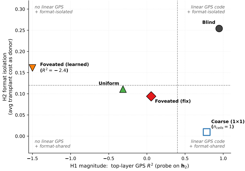
Figure 6: Synthesis: each of the five conditions occupies a distinct (H1 magnitude, H2 format isolation) coordinate. X-axis : top-layer GPS R^2 on \mathbf{h}_2 (foveated (learned) clipped at -1.5 , actual -2.43 ). Y-axis : -1 \times average cross-condition transplant cost when this condition is the donor (higher Y = this condition’s hidden state is more disruptive to other conditions’ policies = more format-isolated as donor). Coarse ( 1 \times 1 ) has only one measured donor cell (coarse \rightarrow blind) and is shown as a hollow marker; the four coarse-recipient cells are pending. The encoder–memory race (H1) is the X axis; H2 format-isolation is the Y axis. Conditions land at distinct coordinates — the H1 ordering is one dimension of a larger picture, not the whole picture.
