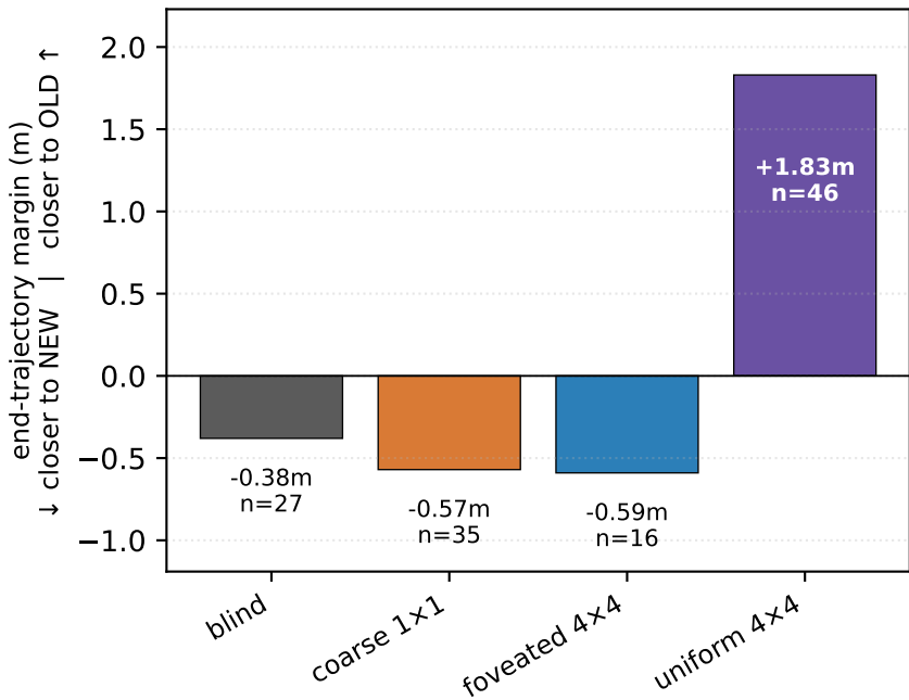
Persistent agent goes to OLD goal — uniform only
