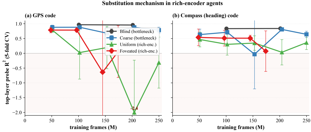
Figure 28: Cross-training probe profile across 4–5 training checkpoints per condition, truncated at 250M frames. (a) Top-layer GPS R^2 . (b) Top-layer compass R^2 . (500 ep/probe, 5-fold CV, single seed; hollow dotted = partial-data ckpts; negative- R^2 outliers clipped at -2.0 .)
