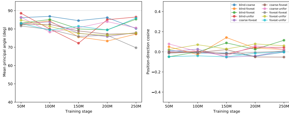
Figure 31: Subspace evolution over training. (a) Mean principal angle between condition-pair top- K subspaces, plotted across five training stages ( \sim 50\text{M} to \sim 250\text{M} frames; sighted at ckpt 10/20/30/40/49, blind at 10/15/20/25). Angles are already [82, 89] at the earliest probed stage and stay near-orthogonal throughout. (b) Position-encoding direction cosines are essentially zero throughout (range [-0.05, +0.14] ), indicating direction divergence is committed before the earliest probed checkpoint. Single seed; 4–5 ckpts per condition.
