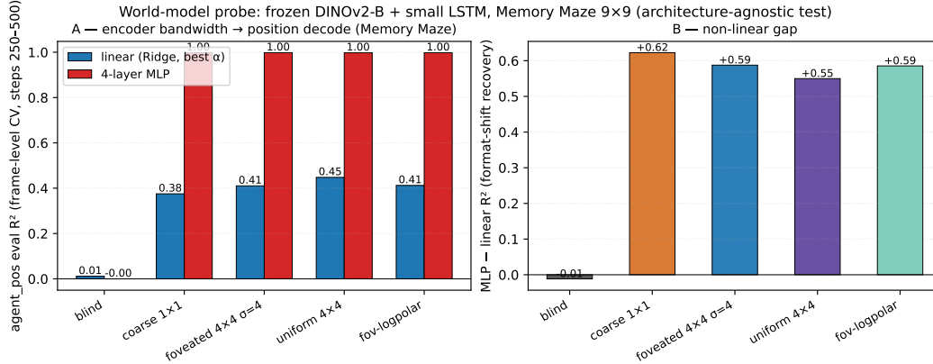
Figure 7: Architecture-agnostic confirmation: format shift reproduces on Memory Maze with a frozen DINOv2-Base + small LSTM stack. (A) Linear (Ridge, best of \alpha \in \{0.1, 1, 10, 100, 1000\} , blue) and 4-layer MLP (red) eval R^2 for agent_pos from the LSTM hidden state, frame-level random CV (80/20), eval window steps 250–500 of T=500 Memory-Maze trajectories. Linear R^2 is monotone-increasing with encoder bandwidth (BLIND 0.01 → UNIFORM 0.45); MLP R^2 saturates at \approx 0.998 for all sighted conditions and is at chance for BLIND. (B) The non-linear gap (MLP–linear) is monotone-decreasing with bandwidth: format-shift recovery is largest where linear readability is smallest (COARSE +0.62 vs. UNIFORM +0.55), the same dichotomy our Habitat agent shows in Figure 2. The opposite linear- R^2 direction relative to Habitat reflects the absence of GPS/compass channels in the Memory-Maze setup — without an alternative positional anchor, the encoder is the only route, and BLIND carries no signal.
