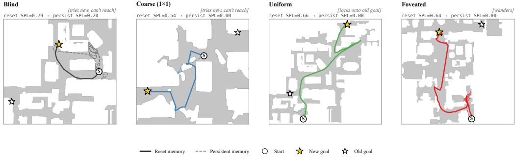
Figure 32: Persistent-memory failure modes — one canonical paired-episode case per condition (extended catalog: Appendix E.6). Aggregate per-condition margin = avg dist(persistent end → old goal) − avg dist(persistent end → new goal) over same-floor failures (reset SPL > 0.5, persistent SPL < 0.2, persistent steps ≥ 30, |\Delta y_{\text{goal}}| < 0.5\text{m} ): Blind −0.38m ( n=27 ), Coarse −0.57m ( n=35 ), Foveated −0.59m ( n=16 ), Uniform +1.83m ( n=46 , closer to OLD goal) . Single seed.
