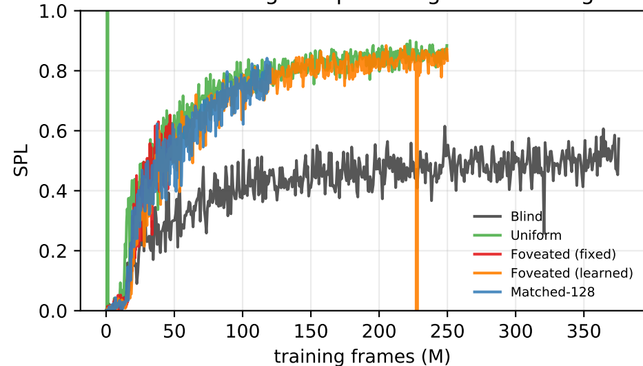
Success-weighted path length vs. training
