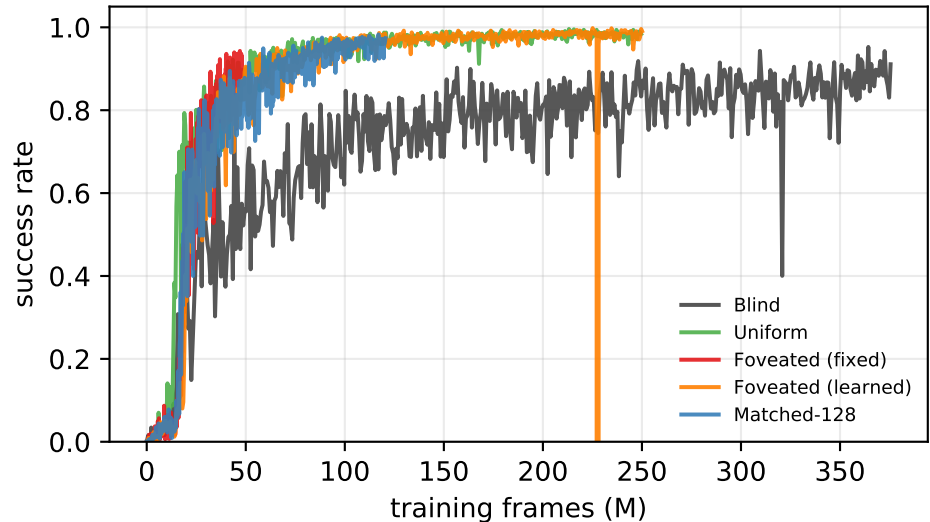
Success rate vs. training
