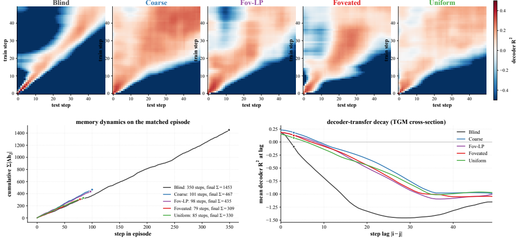
Figure 4: Temporal format: blind-vs-sighted dichotomy and within-sighted spectrum across three quantitative views. Top row: step-by-step generalisation of a linear goal-vector decoder. Each 50 \times 50 heatmap shows decoder R^2 when fit at step i (row) and evaluated at step j (column). A diagonal-only structure (blind) signals a step-by-step rotating basis: the decoder at step t does not transfer to step t \pm 30 . A square-block structure (coarse) signals a stationary readout. Sighted-rich conditions interpolate. Bottom row, left: cumulative memory displacement \Sigma|\Delta h_2| vs step-in-episode on the matched episode (Almena, episode 157; same start, same goal, all five conditions complete it), one curve per condition. Blind’s curve ends at 1453 over 350 winding steps; sighted conditions stop early at 309–467 over 79–101 direct steps (foveated 309 < \text{uniform } 330 < \text{fov-LP } 435 < \text{coarse } 467 ). Right: mean decoder R^2 as a function of step lag |i - j| — each top-row TGM heatmap collapsed to a single curve. The five curves fan out monotonically: blind drops to \approx -1.2 (catastrophic transfer); coarse holds R^2 \approx +0.18 at small lag (strongest stationary block); fov-LP +0.13 , foveated +0.13 , uniform +0.08 . The within-sighted ranking inverts encoder bandwidth: less bandwidth, more stationary readout. Per-unit autocorrelation \tau values (Murray [Murray et al., 2014]) and a persistent-homology corroboration [Gardner et al., 2022] are reported in Appendix F.
