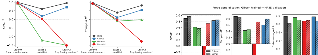
(a) Per-LSTM-layer GPS / compass probe R^2 across all three layers, all four conditions (single train/test fit; the 5-fold CV mean reported in Table 1 matches qualitatively but with different magnitudes for rich-encoder conditions). Compass tells the same story as GPS at smaller magnitude.
