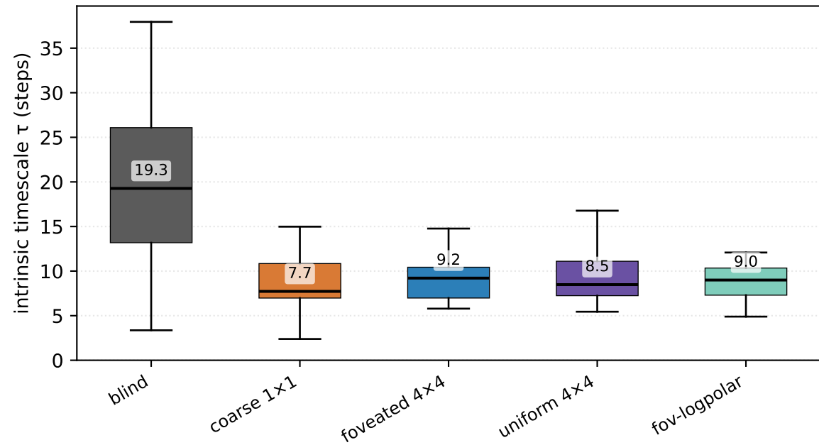
Murray 2014 intrinsic timescale: blind 2.1× longer than sighted
