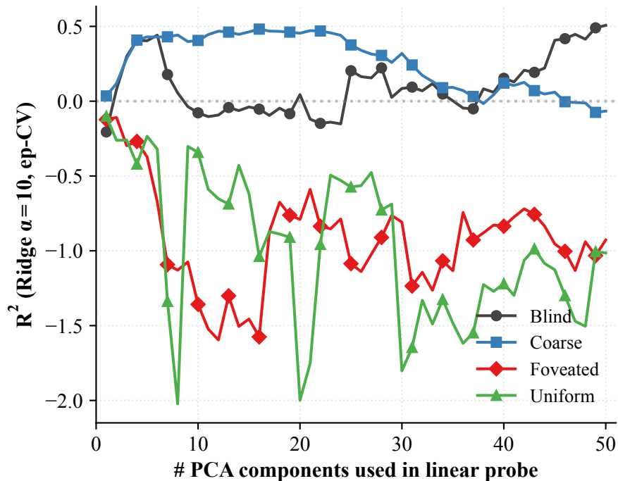
(a) Linear readout vs # PCs used Why ID \sim 3 across conds but linear R^2 differs: position is embedded along DIFFERENT manifold directions (Blind saturates fast \rightarrow linear axis; Uniform rises slowly \rightarrow distributed)
