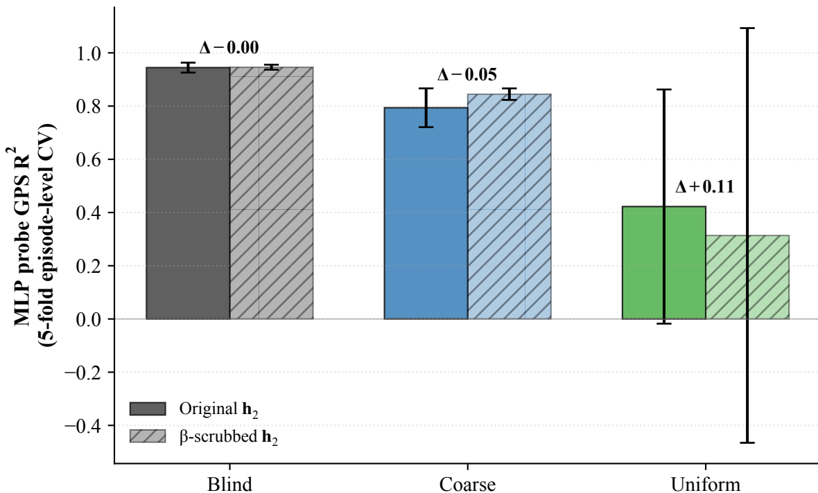
F3: GPS-subspace scrubbing — does removing the linear \beta direction kill MLP-recoverable position? (foveated deferred to 250M re-probe)
