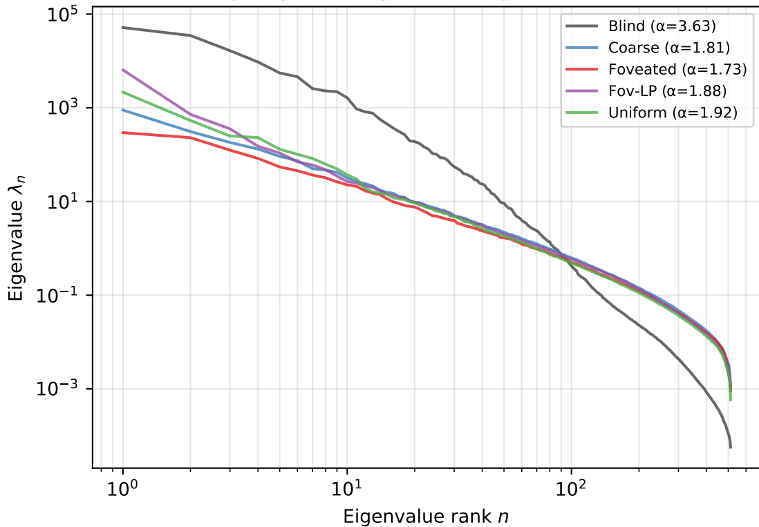
Eigenspectrum power law per condition
