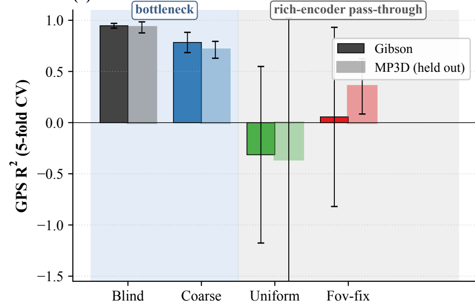
(a) Bottleneck retains GPS
