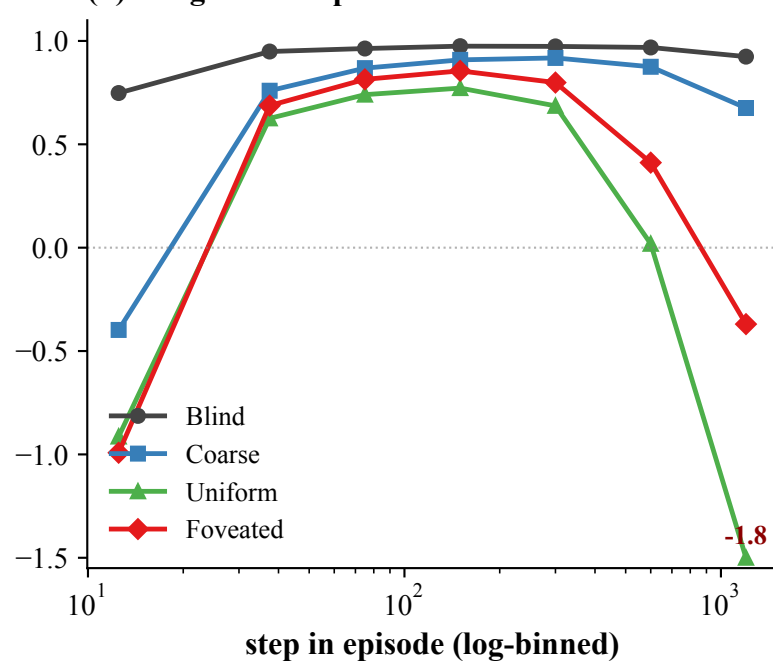
(b) Long-tail collapse
