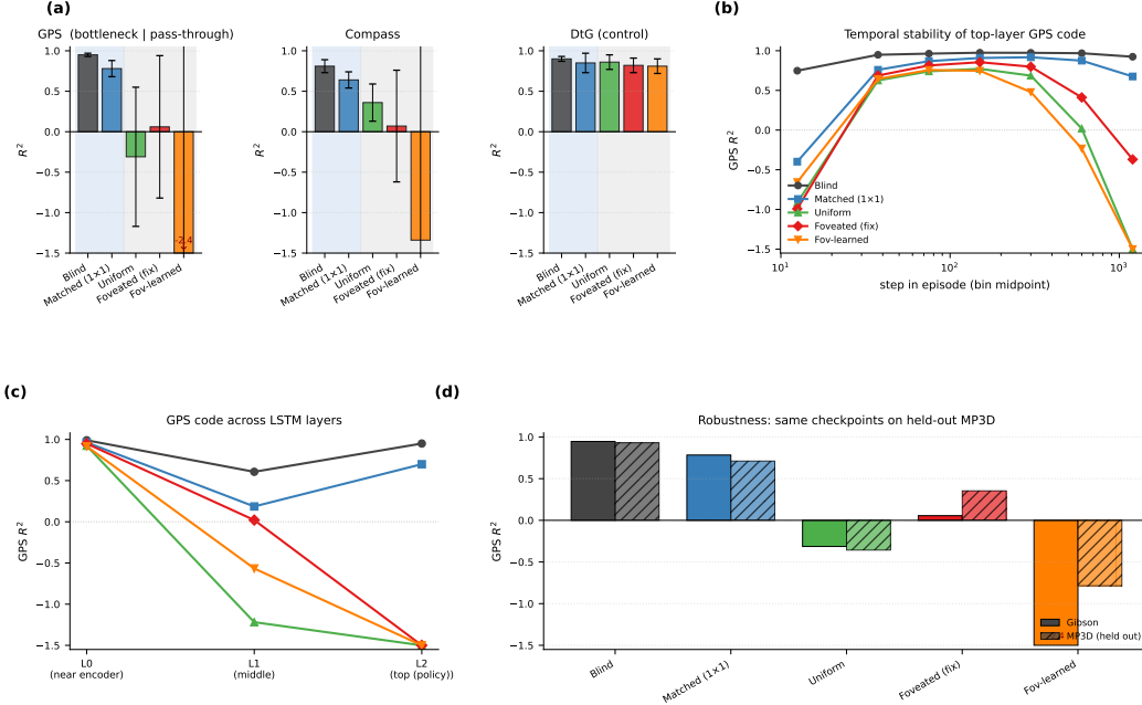
Figure 2: H1 evidence in one figure. (a) Current-state probe R^2 (5-fold CV, Ridge \alpha = 10 , full-length deterministic rollouts) for GPS, compass, and DtG. Blind and matched-compute (the bottleneck conditions) decode world-frame GPS / compass robustly; uniform / foveated / foveated-learned do not. DtG decodes everywhere because every agent must track it. (b) Top-layer GPS R^2 binned by step-in-episode (out-of-fold prediction): all five conditions encode top-layer GPS in the typical-episode window (steps \sim 25 –200), and the rich-encoder conditions then overwrite the code (negative R^2 in the long-tail 800+ bin), while bottleneck conditions hold R^2 > 0.7 to step 800+. The headline “rich-encoder \approx chance” in panel (a) is therefore primarily long-tail behaviour. (c) Per-LSTM-layer GPS R^2 (no-cap, single-fit on top-layer hidden states): all five conditions have GPS at Layer 0 (where the GPS sensor embedding enters the LSTM input vector — this lower-bound is at least partly a sensor-pass-through effect, not the network “computing” position); the divergence is at Layer 2, the policy readout. (d) Same checkpoints, evaluated on held-out MP3D (300 episodes/condition, deterministic protocol). The bottleneck-vs-pass-through ordering is preserved; foveated does recover to a mild positive ( R^2 = +0.35 ) on MP3D, consistent with Gibson-specific feature use by the foveated encoder.
