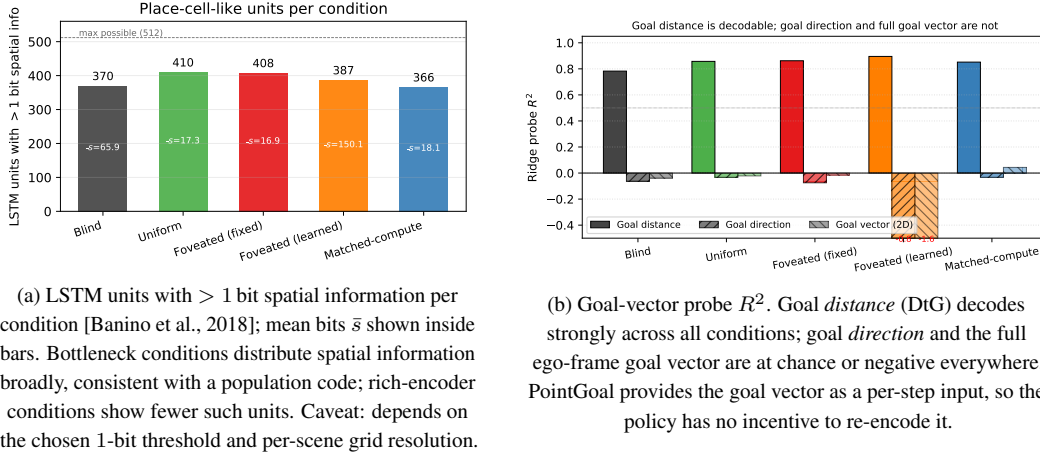
Figure 6: Population-coding indicator and goal-vector probe (referenced from §4.6).
