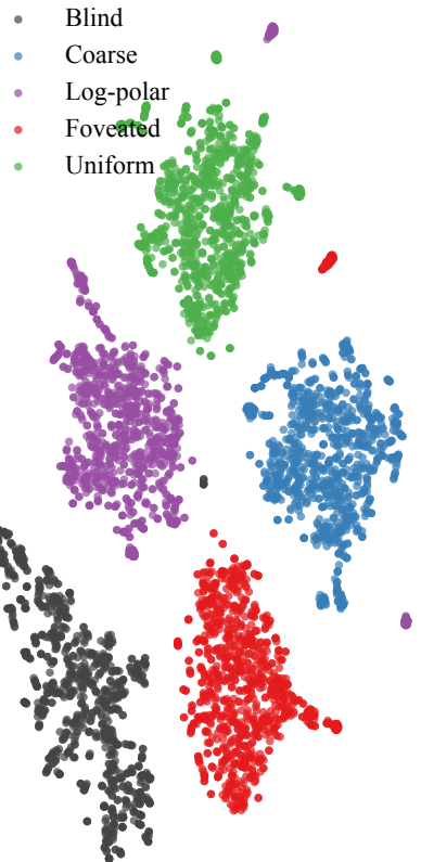
Joint t-SNE (5 conditions pooled)
