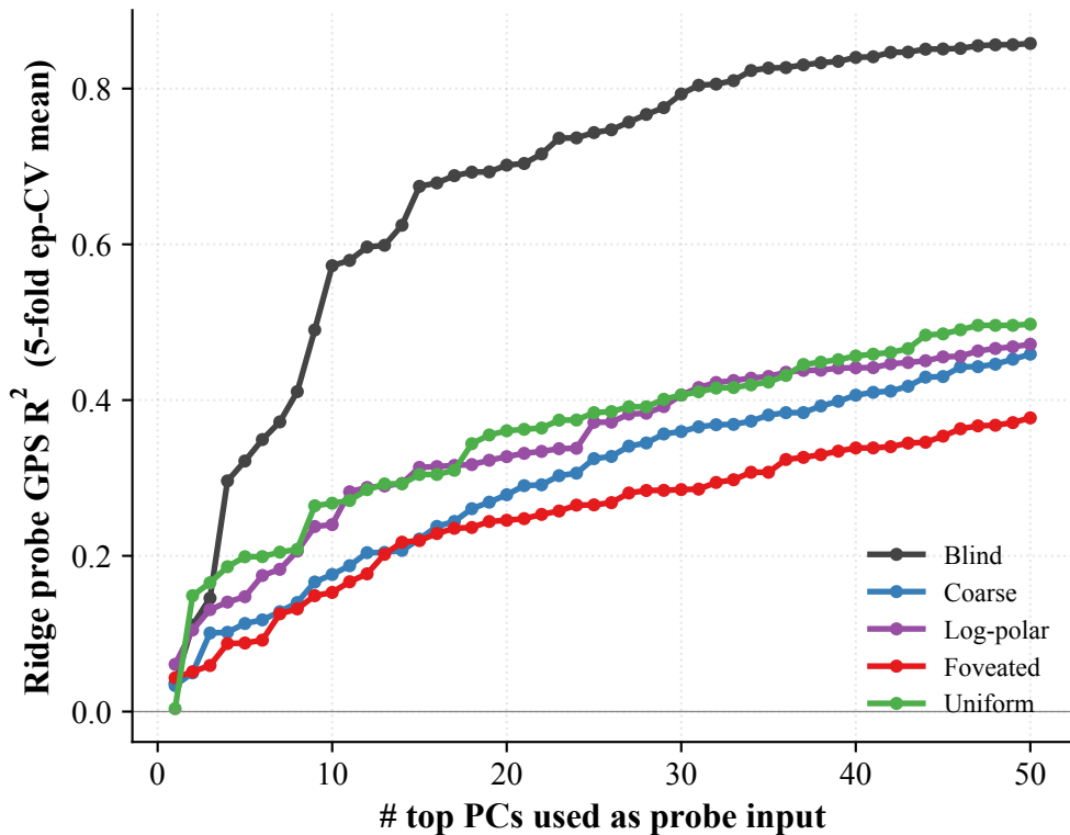
Linear readout vs. \# PCs
