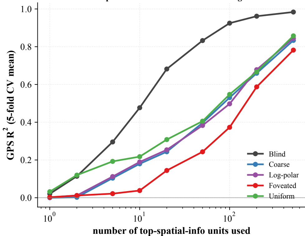
Sparse-vs-distributed GPS decoding
