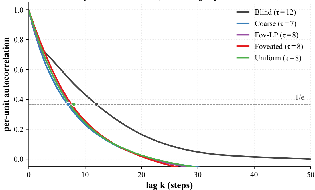
Murray intrinsic timescale (1/e-crossing of per-unit autocorr)
