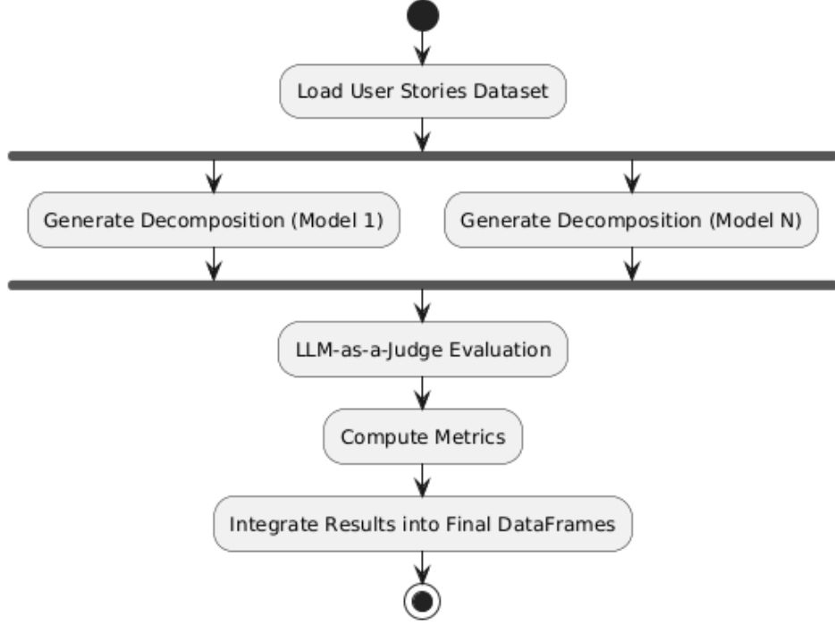
Figure 1 UML activity diagram of the LocalLLM-DataForge framework.
