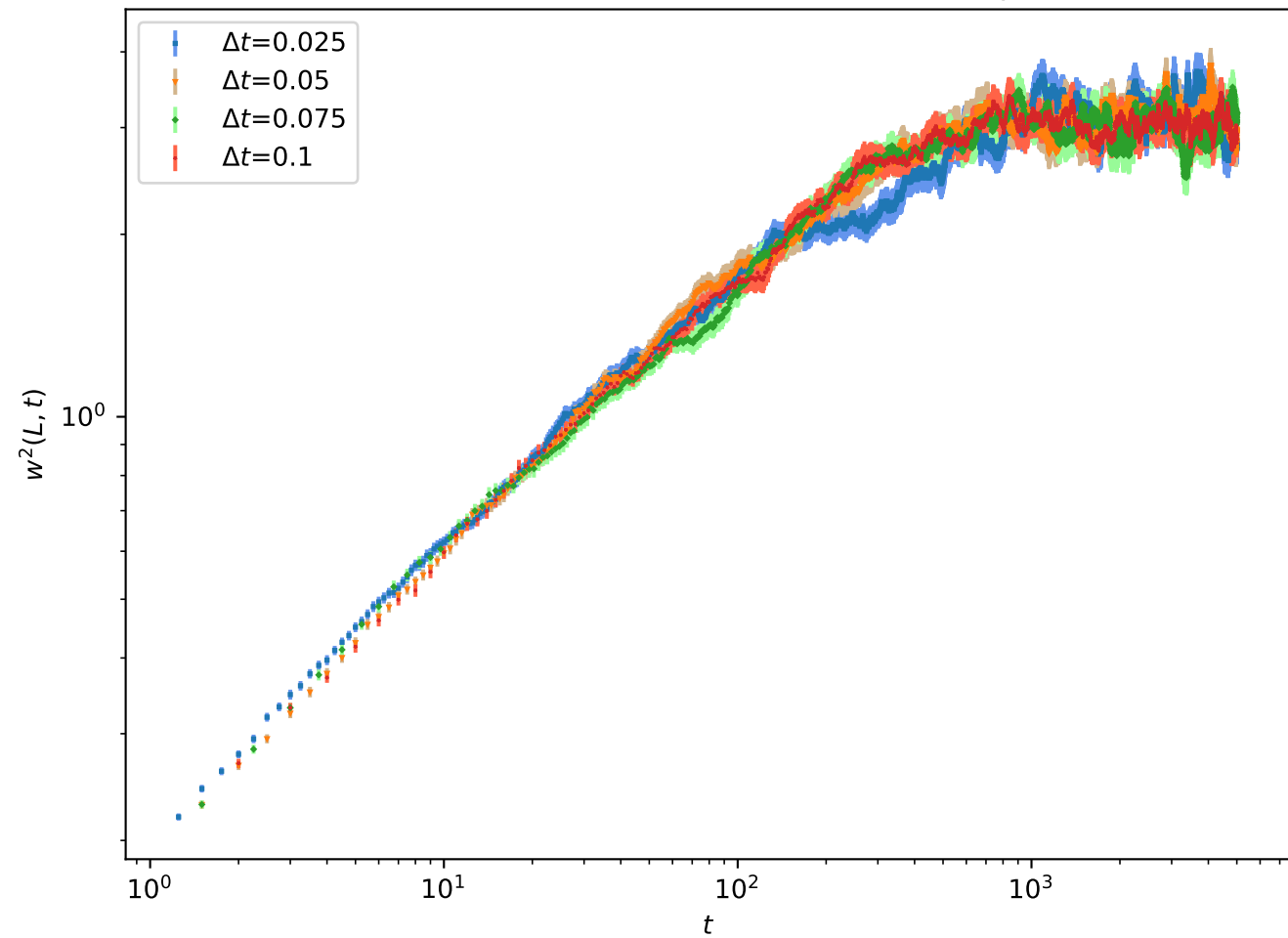
Width of the surface, variable time step
