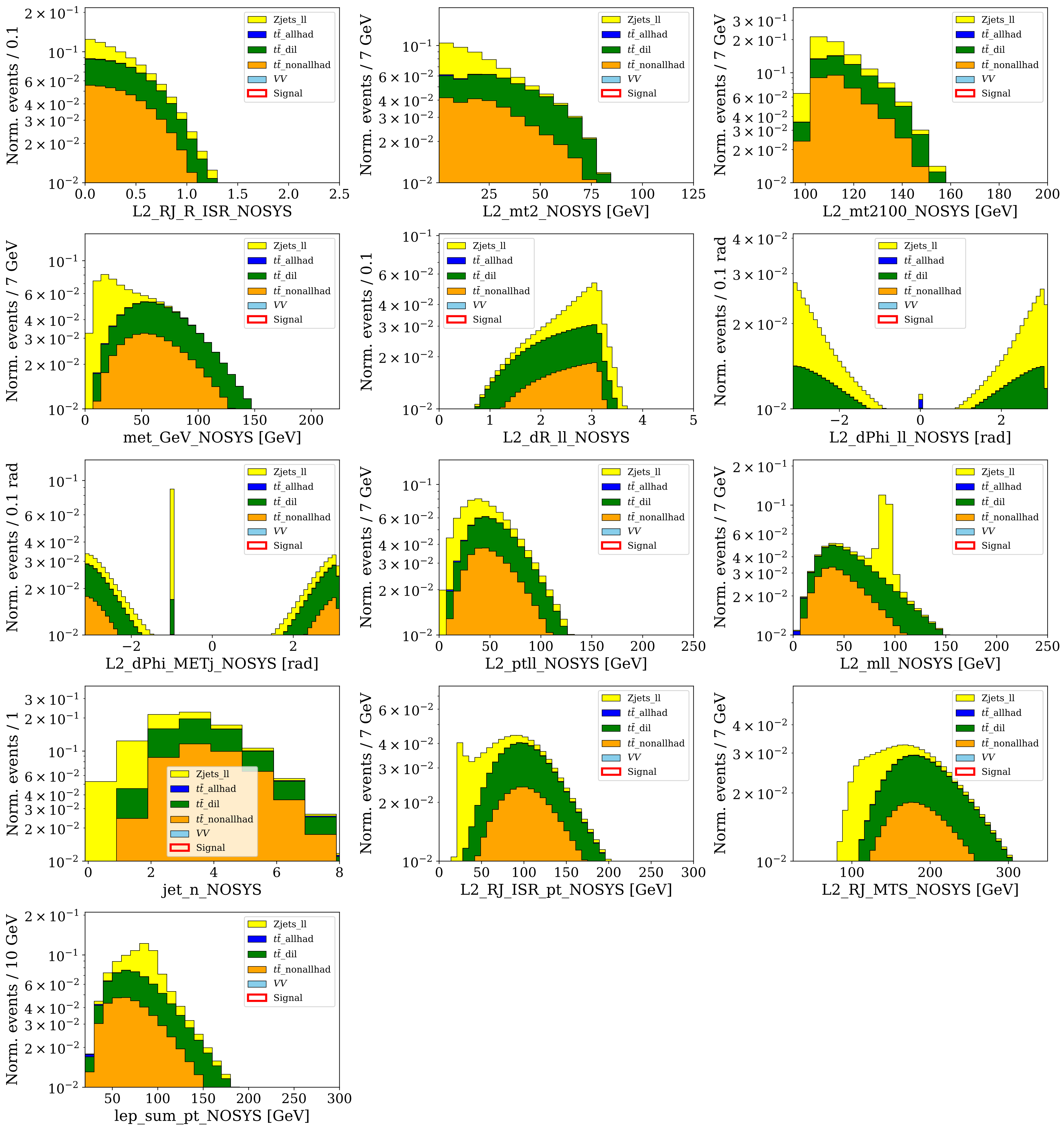
C1N2_WZ_2L signal vs SM bkg / Normalised to bkg
