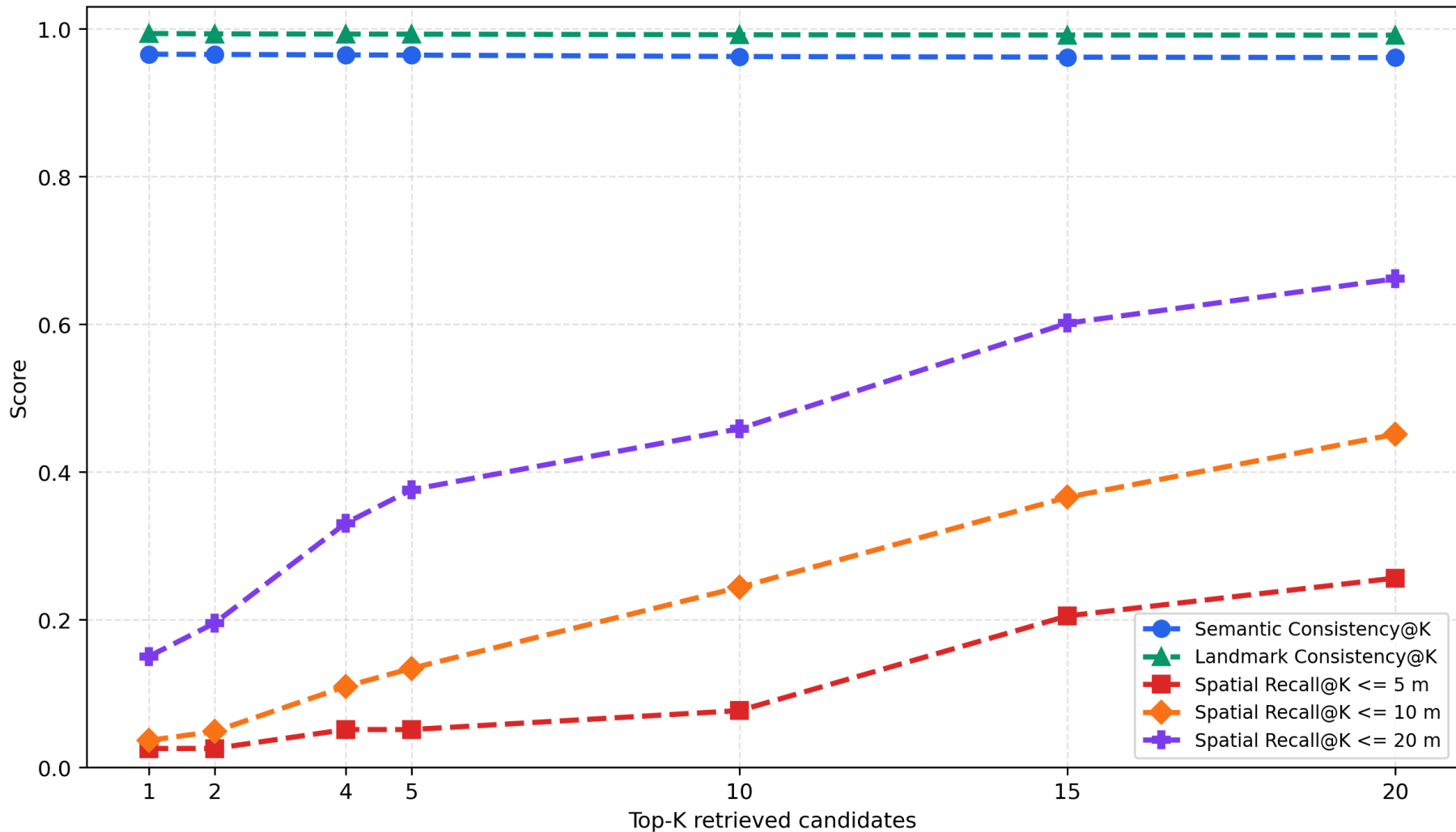
Sequence 08: Our Descriptor Consistency vs. Spatial Recall
