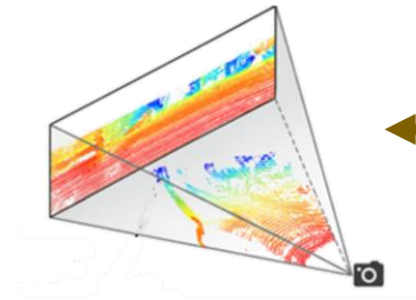
Spherical projection
