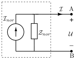
Equivalente Norton
