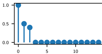
y = (1 + .5L + .4L^2)w
