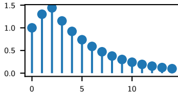
(1 - .8L)y = (1 + .5L + .4L^2)w
