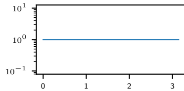
spectrum (log scale)
