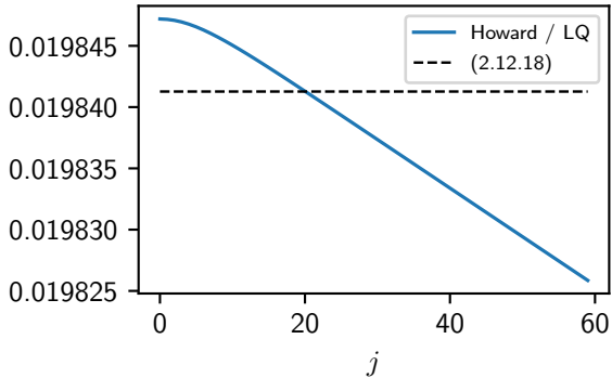
response of c_{t+1+j}
