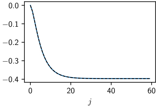
response of b_{t+1+j}
