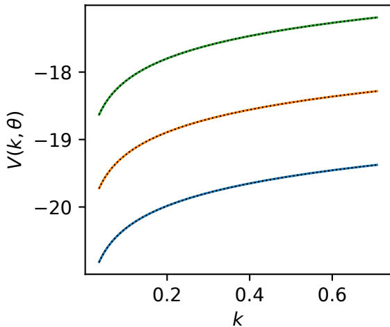
value (dotted: closed form)
