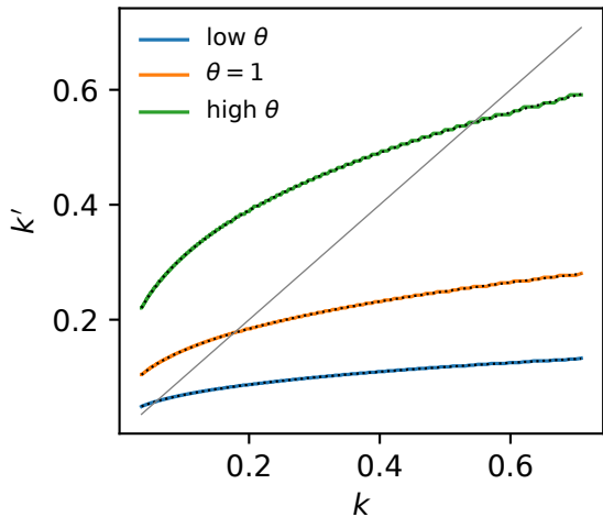
policy (dotted: \alpha\beta y )
