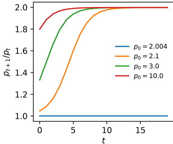
equilibrium inflation paths
