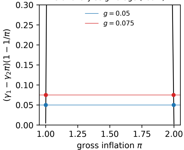
stationary seigniorage (zoom)
