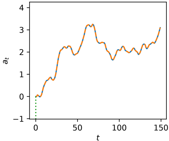
assets (Ponzi path: a_t \rightarrow -\infty , off scale)
