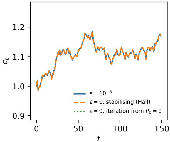
consumption (Ponzi path: c = b , off scale)
