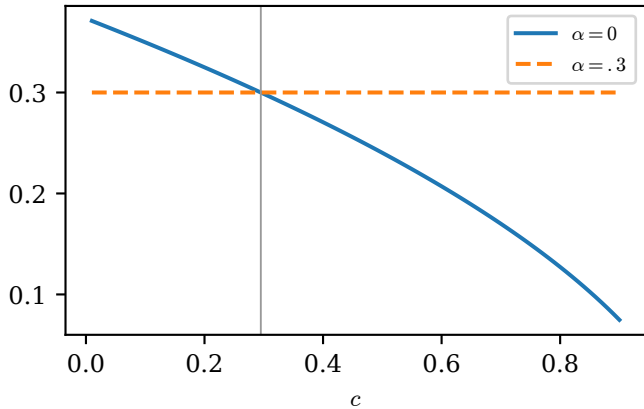
hazard 1 - F_\alpha(\bar{w}^-)
