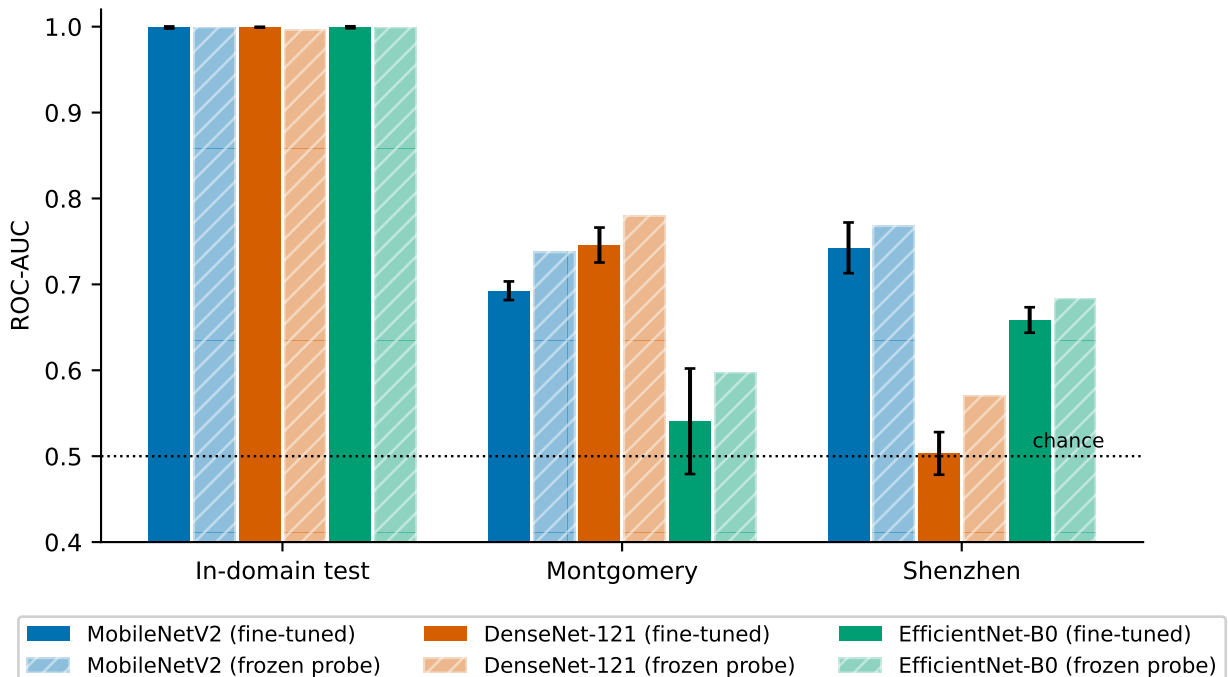
External generalisation by backbone (raw input)
