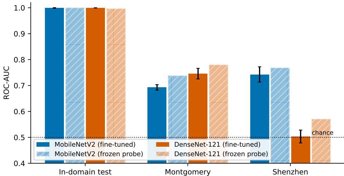
External generalisation by backbone (EfficientNet-B0 pending)
