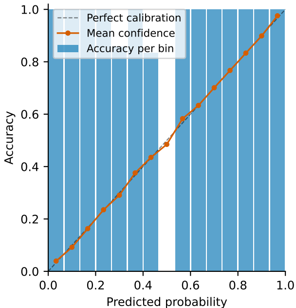
Before scaling (ECE 0.770)
