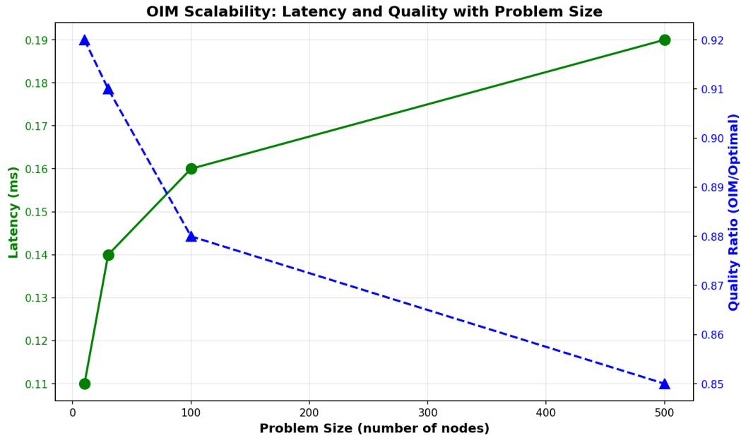
Figure 7.2: OIM latency and solution quality as functions of problem size. The sub-linear latency growth indicates practical scalability to very large problems. Quality ratio degrades gracefully with problem size.
