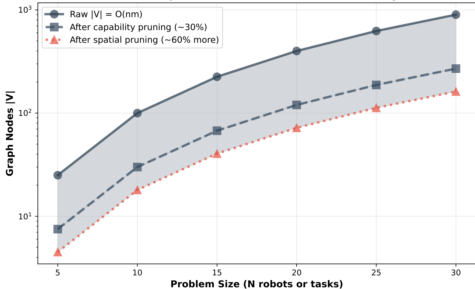
Scalability: Effective Node Reduction via Pruning
