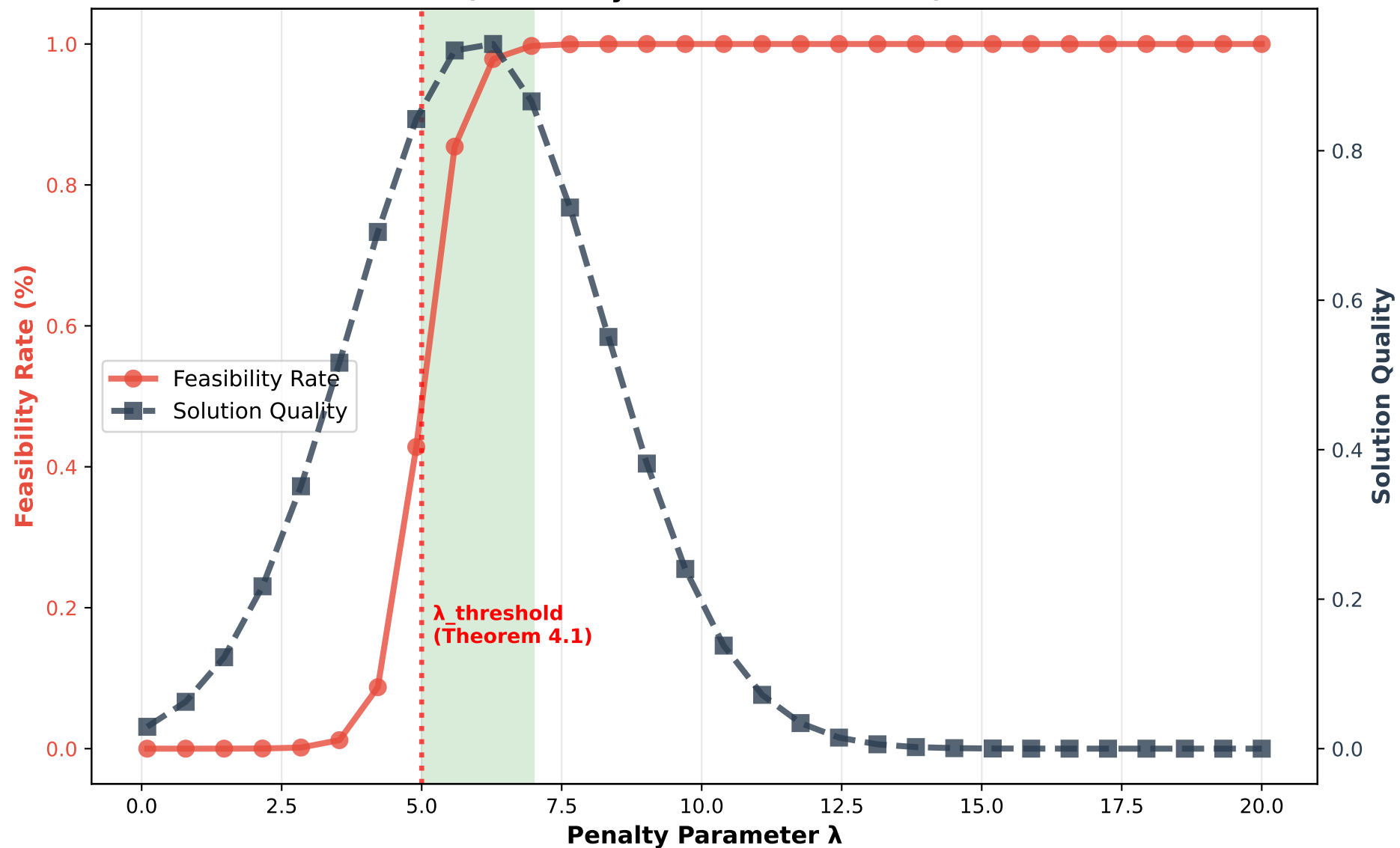
MWIS Quality vs Penalty Parameter \lambda (Feasibility Guarantee Trade-off)
