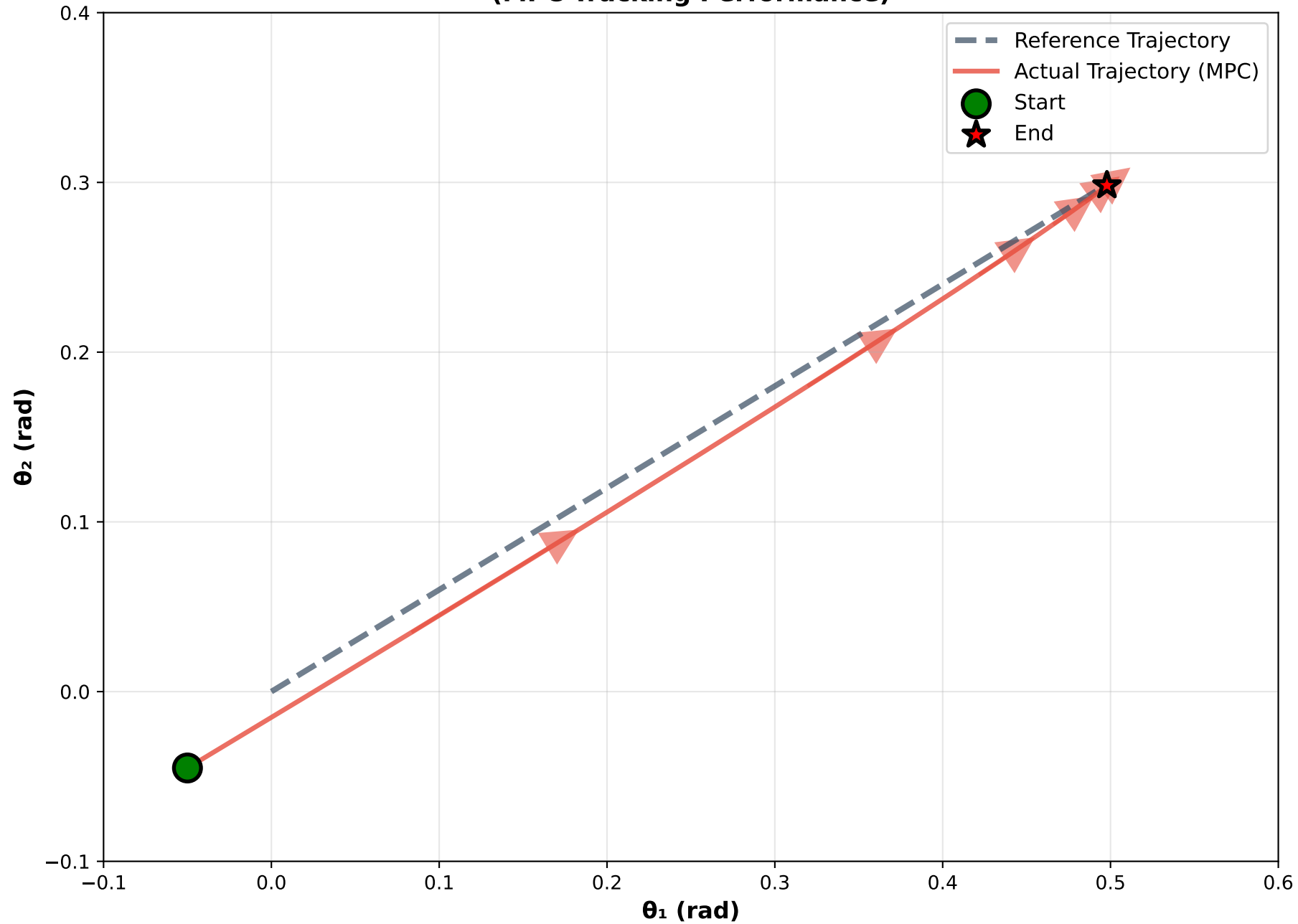
Phase-Space Trajectory: 2-DOF Arm Configuration Space (MPC Tracking Performance)
