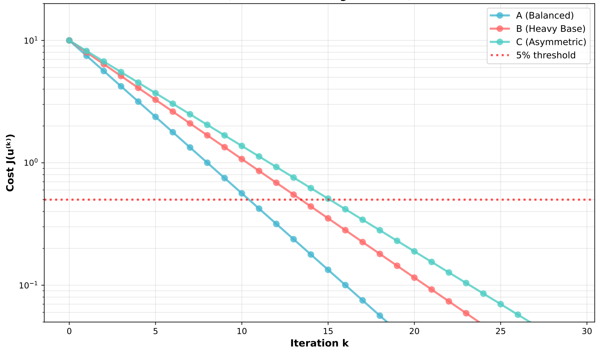
PIPG Convergence: All Three Robot Cases (Geometric Convergence Rate)
