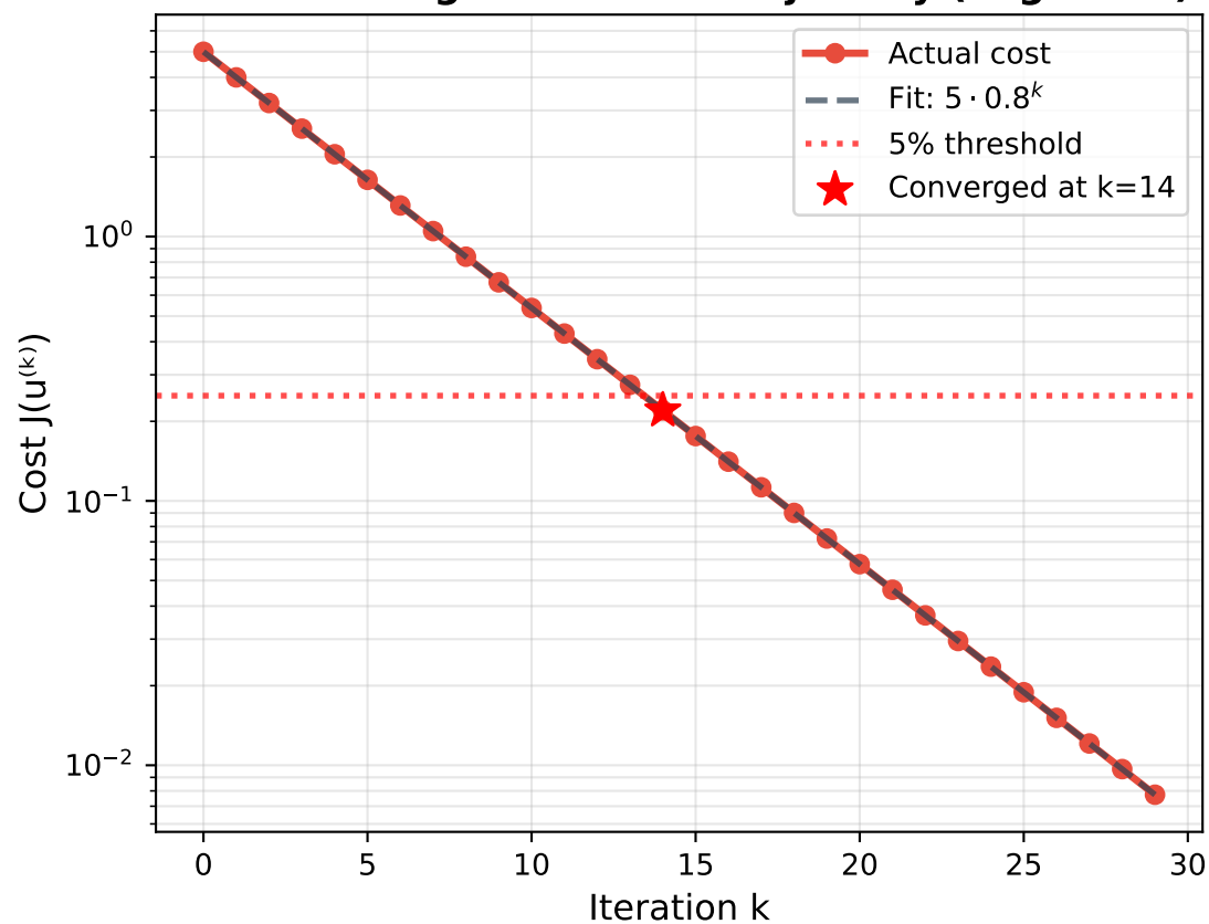
PIPG Convergence — Full Trajectory (Log Scale)
