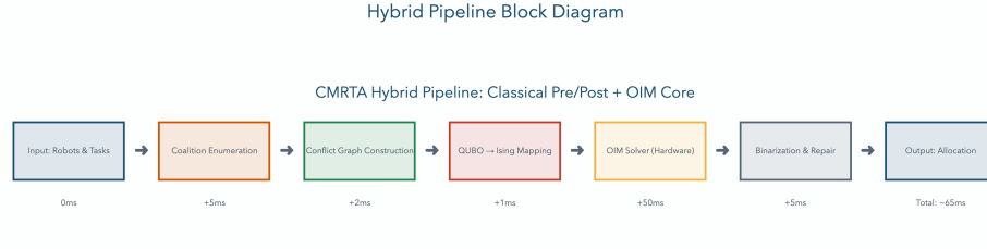
Figure 5.5: Hybrid Pipeline Block Diagram. Pre-processing (classical): enumerate feasible coalitions, build conflict graph, compute utilities. OIM solve: physical system minimizes Hamiltonian, returns binary phases. Post-processing: convert phases to allocation, check feasibility, repair any constraint violations via greedy heuristics.
