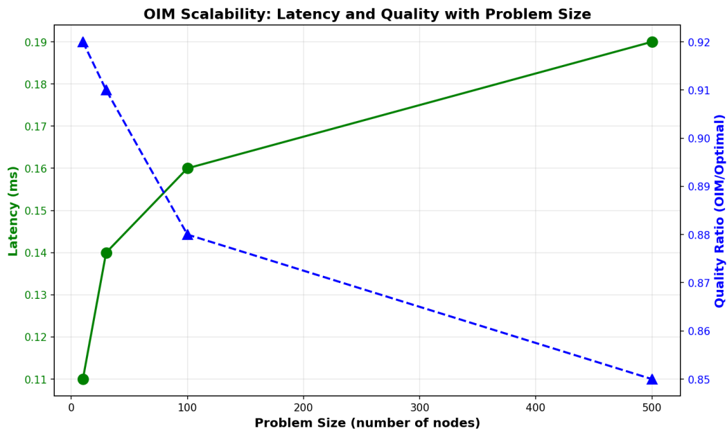
Figure 7.2: OIM latency and solution quality as functions of problem size. The sublinear latency growth indicates practical scalability to very large problems. Quality ratio degrades gracefully with problem size.
