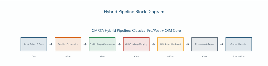
Figure 5.6: Hybrid Pipeline Block Diagram. Pre-processing (classical): enumerate feasible coalitions, build conflict graph, compute utilities. OIM solve: physical system minimizes Hamiltonian, returns binary phases. Post-processing: convert phases to allocation, check feasibility, repair any constraint violations via greedy heuristics.
