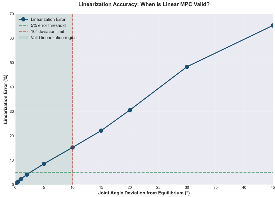
Figure 6.1: Linearization Accuracy: Deviation vs. Error. Shows how linearization error grows with joint angle deviation from equilibrium. Green shaded region indicates the valid linearization zone ( |\Delta\theta| < 10^\circ with error < 5\% ). Red vertical line marks the 10^\circ deviation limit beyond which nonlinear effects dominate. This plot validates our choice of linear MPC for near-equilibrium trajectory tracking in robotics applications.
