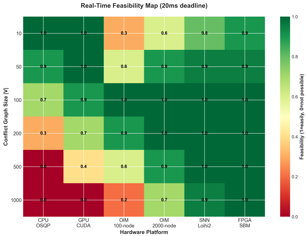
Figure 7.5: Heatmap showing feasibility of different hardware platforms for various MRTA problem sizes under 20 ms real-time deadline. Green cells indicate easily feasible configurations; yellow cells show marginal feasibility; red cells indicate infeasible (exceeds deadline). The map guides hardware selection for given problem scales.
