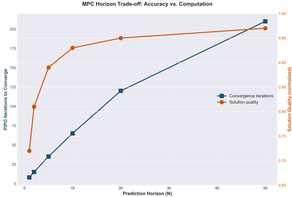
Figure 6.2: MPC Horizon Trade-off: Accuracy vs. Computation. Left y-axis (blue): PIPG iterations required to converge as a function of prediction horizon N . Right y-axis (orange): normalized solution quality. The figure shows that longer horizons ( N > 10 ) provide diminishing returns in quality while significantly increasing computational cost. N = 5 offers a good balance for real-time robotics applications with tight latency constraints.
