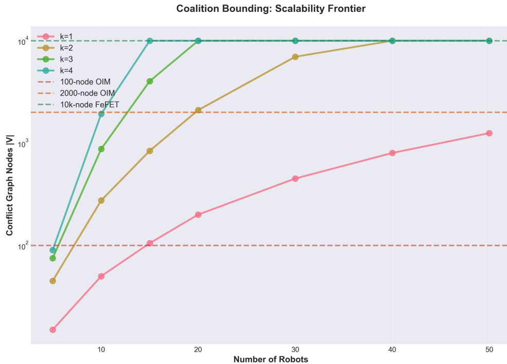
Figure 5.5: Coalition Size vs. Hardware Nodes: Scalability Frontier. Shows how the number of conflict graph nodes scales with the number of robots for different maximum coalition sizes k = 1, 2, 3, 4 . Horizontal dashed lines indicate hardware feasibility regions: 100-node OIM (red), 2000-node OIM (orange), 10k-node FeFET (green). The feasibility window shows realistic problem sizes that fit current hardware.
