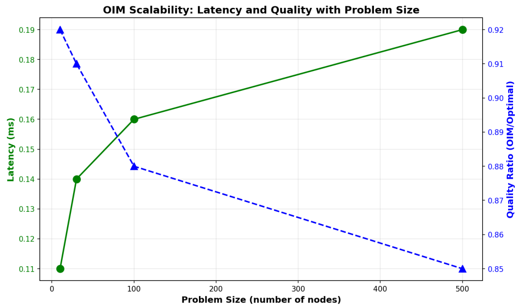
Figure 7.2: OIM latency and solution quality as functions of problem size. The sub-linear latency growth indicates practical scalability to very large problems. Quality ratio degrades gracefully with problem size.
