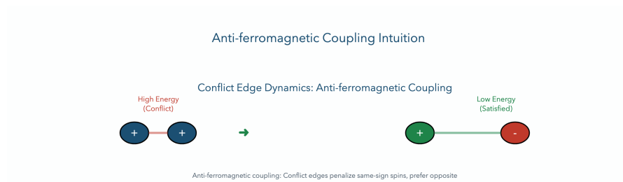
Figure 5.6: Anti-ferromagnetic Coupling Intuition. (a) Two oscillators with positive coupling: prefer same phase (both at 0 or both at \pi ). (b) Two oscillators with negative (anti-ferromagnetic) coupling: prefer opposite phases (one at 0, one at \pi ). This is the conflict constraint: “at most one can be selected.”
