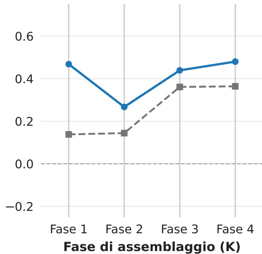
MCC
