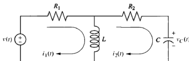
Figure 1: An RLC circuit
