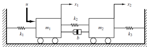
Figure 2: Mass spring damper mechanical system
