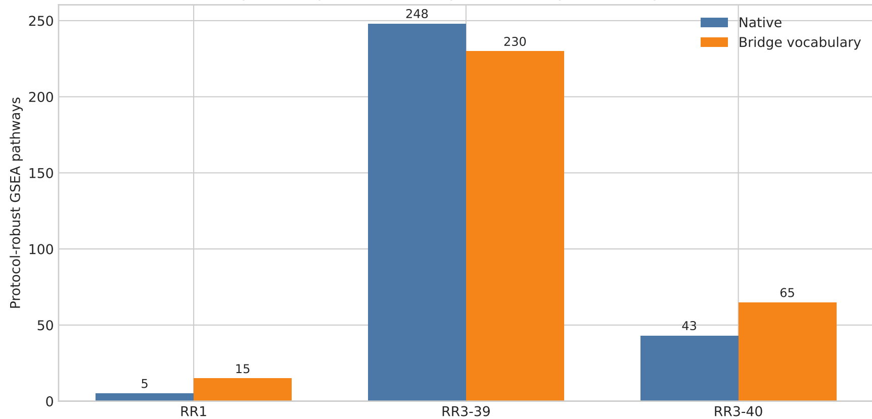
Pathway recovery is not uniformly increased by vocabulary restriction
