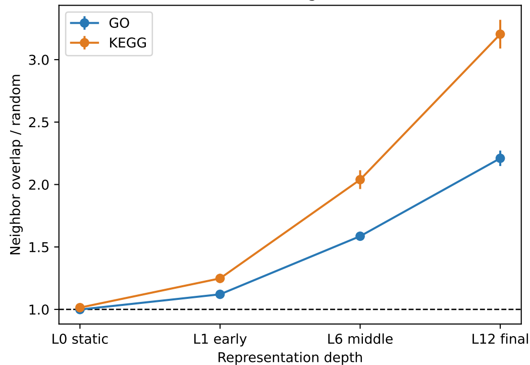
Functional nearest-neighbor enrichment
