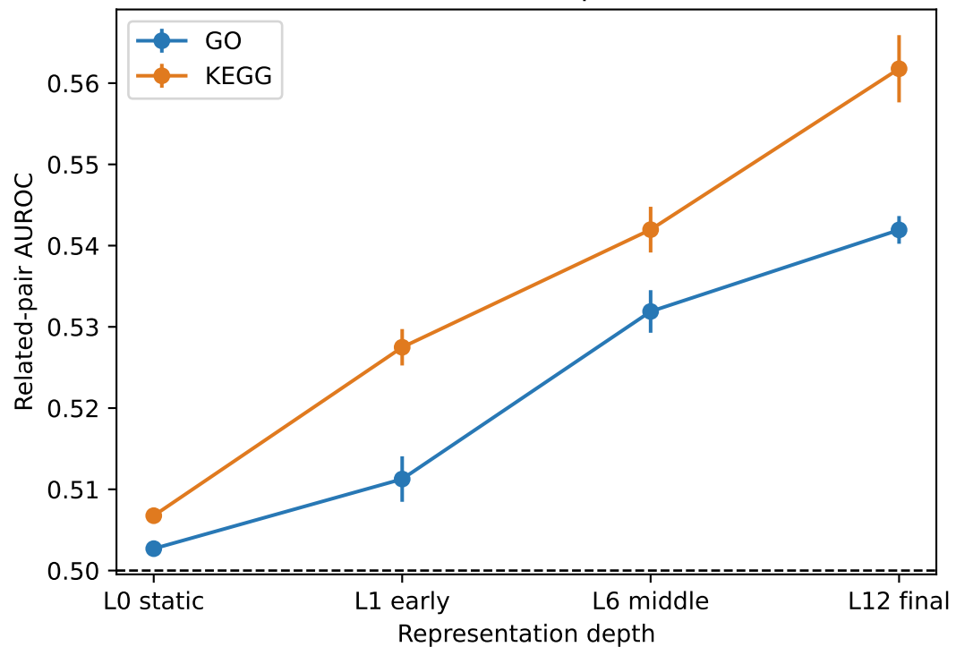
Known relationship retrieval
