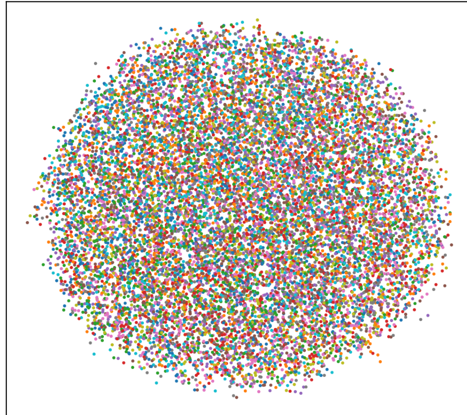
LayerNorm — UMAP
