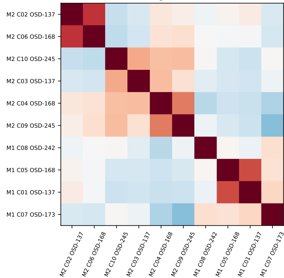
15,165-gene PCA111
