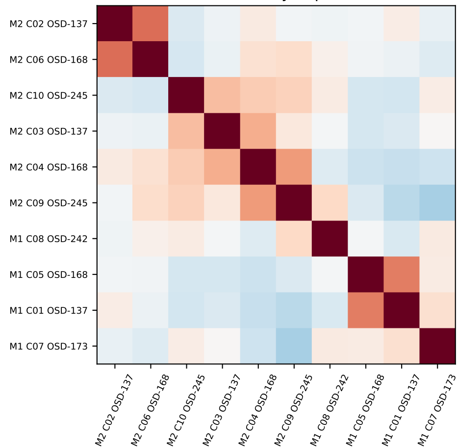
15,165-gene PCA20
