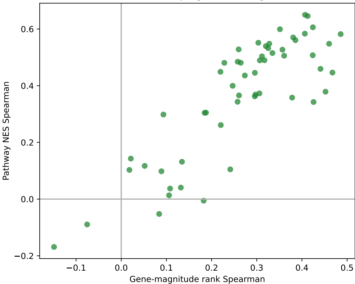
Gene-level versus program-level agreement
